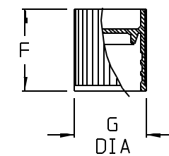
CLOSURE DETAILS
